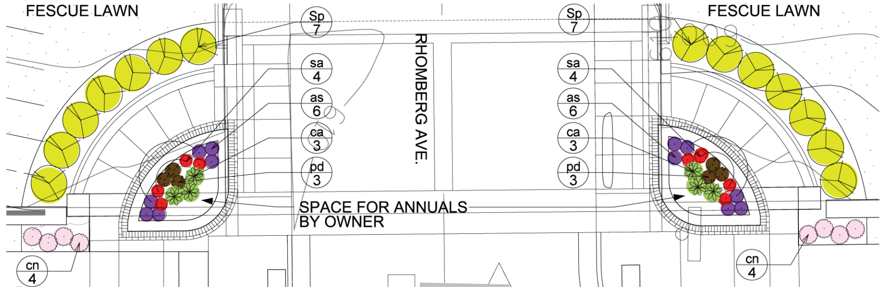
2 RHOMBERG BRIDGE NORTH PLANTING PLAN C738 1/4" = 1'-0" on 22x34 sheet
