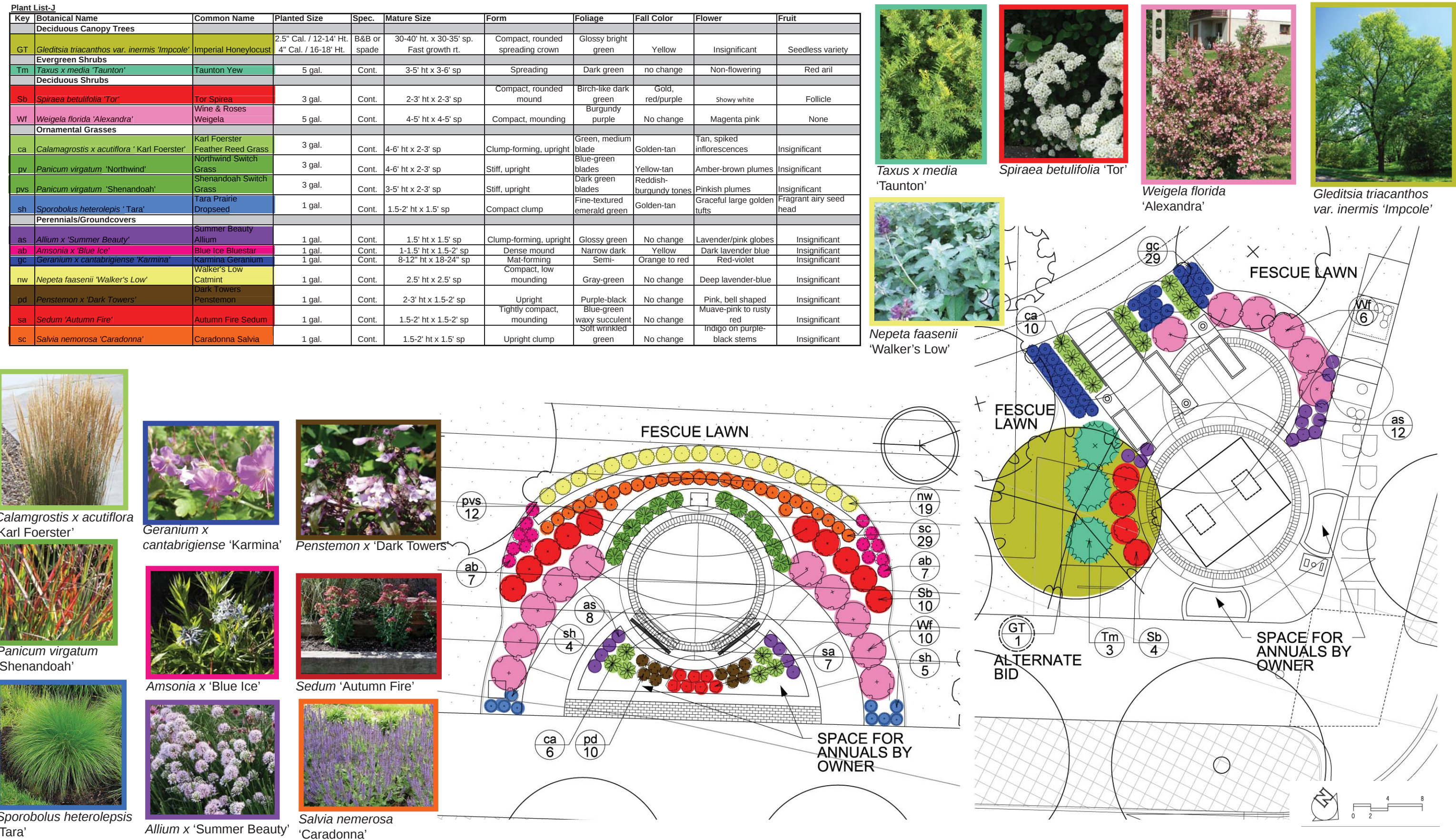
J. 24TH STREET BIKE TRAILHEAD AND OVERLOOK - PLANTING PLAN
